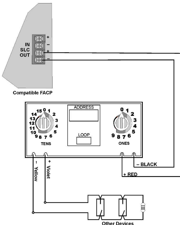
Wiring the HFS-MM
