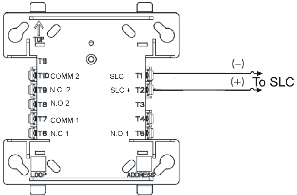
Relay Module wiring diagram
